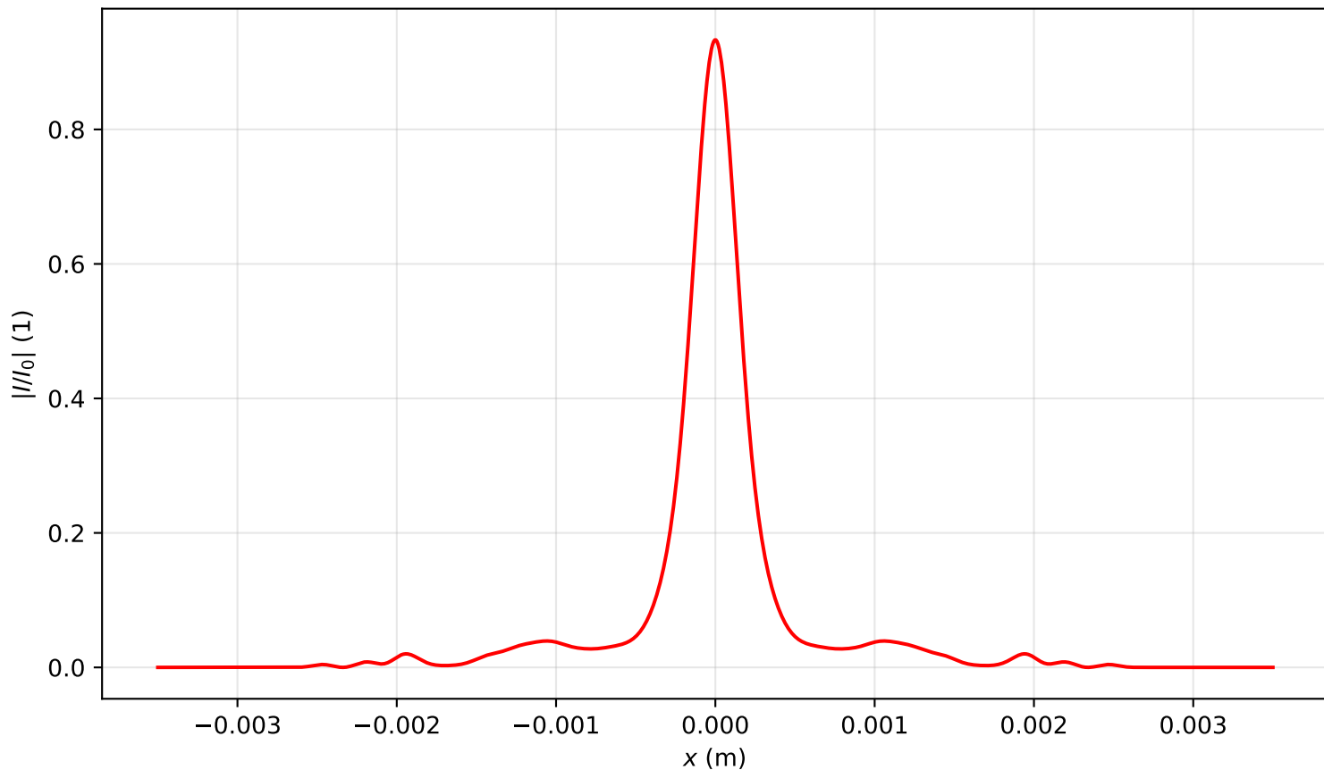
Intensity profile I(x, y = 0, z = 3.105)/I_0 , P_{in}=4.5P_{cr} , artificial time
